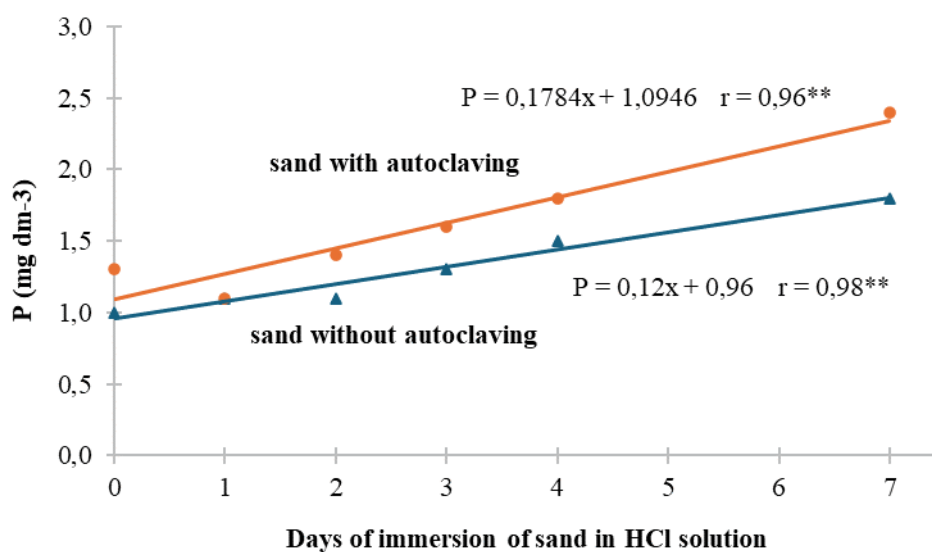
Figure 1 - Phosphorus content in sand after washing with 3% HCl at different immersion periods, including washings with water before and after mixing the sand with the acid solution (experiment 2).
